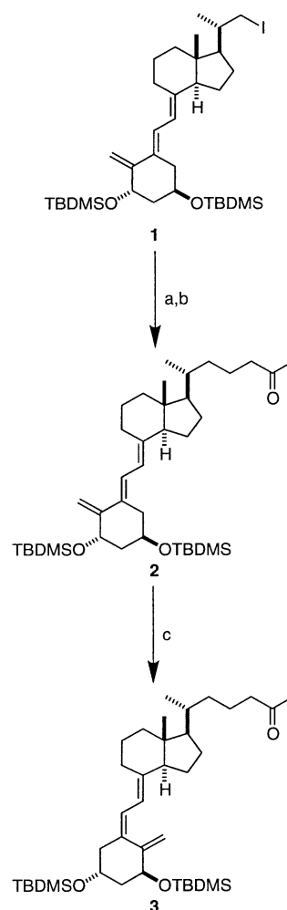
Scheme 1. (a) Prepare methyl vinyl ketone, NiCl 2 ·6H 2 O, Zn dust, pyridine, 65 °C, 30 min; (b) then 1 , pyridine, THF, rt, 2 h, dark; (c) 9-acetylanthracene, TEA, toluene, hv, 10 °C, 15 min. Overall yield 38%.
