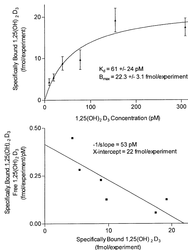
Figure 1. Top: Plot of specific ^{11}\text{C} -1,25(OH) _2 D _3 binding in rachitic chick purified VDR versus 1,25(OH) _2 D _3 concentration. The curve shown is a fit as described in the experimental section from which K_d and B_{\max} were derived. Error bars represent the standard error of the mean ( n=3 ). Bottom: Scatchard plot of the ratio of specifically bound radiotracer to free radiotracer versus specifically bound radiotracer. The line shown is a linear regression fit. The values -1/\text{slope} and X-intercept are shown for comparison, respectively, to K_d and B_{\max} obtained using non-linear regression.
