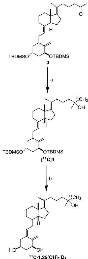
Scheme 3. (a) [ ^{11}\text{C} ]methyl iodide, butyllithium, -70 to -10^\circ\text{C} , 10 min; (b) TBAF, THF, 105^\circ\text{C} , 3–5 min.
