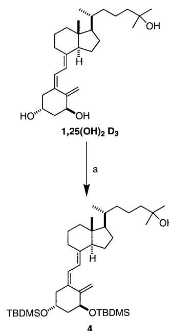
Scheme 2. (a) TBDMSCl, imidazole, DMF, rt, 1 h. Yield 80%.
